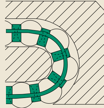
Figure 2 Ball circulating section
