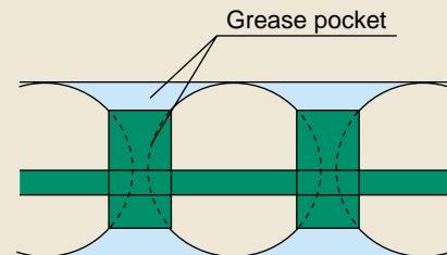
Figure 3 Grease pocket
