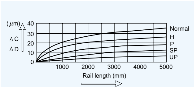
Figure 12 LM rail length and running parallelism
