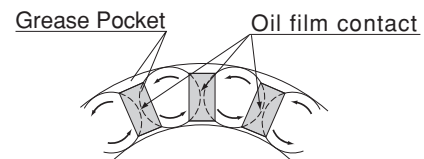
Caged-ball technology
