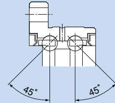
Structure of Support Bearing Model BNS-A
