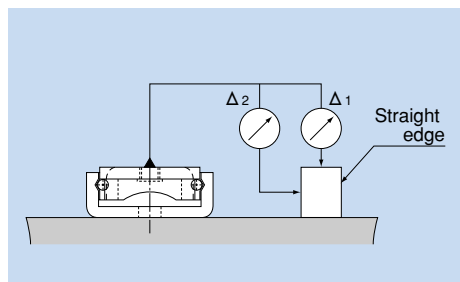
Fig. 3 Method for Measuring Running Straightness
